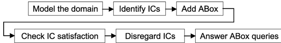
Fig. 1. Using knowledge bases with integrity constraints.
